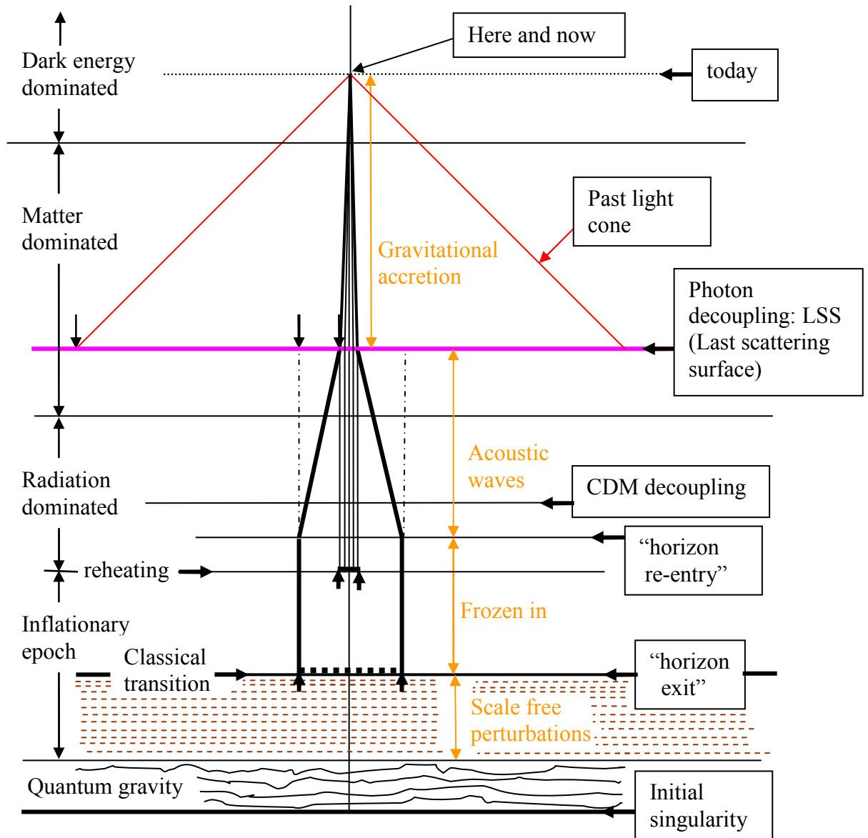
The three downwards pointing arrows on the LSS (photon decoupling) show (left to right) the size of the visual horizon, and the comoving size of the effective domain of influence between the start of the inflationary era to horizon re-entry in the radiation dominated era, and at decoupling of matter and radiation (NB: not to scale!). The two inner upward pointing arrows show the size of the matter horizon at the origin of the MW matter when reheating takes place at the end of inflation.
