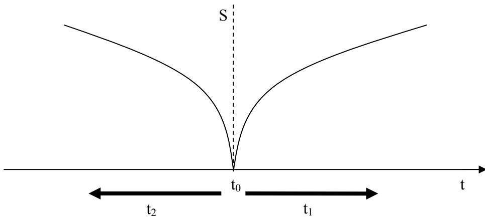
FIGURE 2: THE PAST CONDITION AND THE ARROW OF TIME
