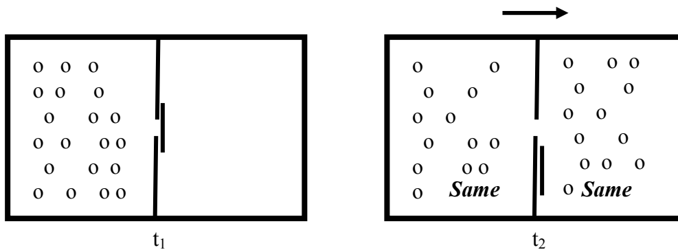
Figure 1a: initial state
