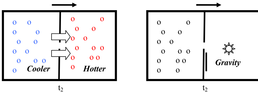
Figure 1c: final state with a gate that only lets through high speed molecules (Maxwell's Demon)
